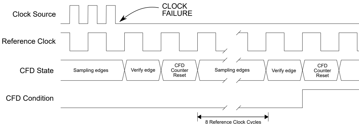
Figure 12-4. Clock Failure Detection (CFD) Timing Diagram
