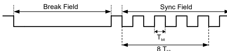
Figure 25-9. Auto-Baud Timing
