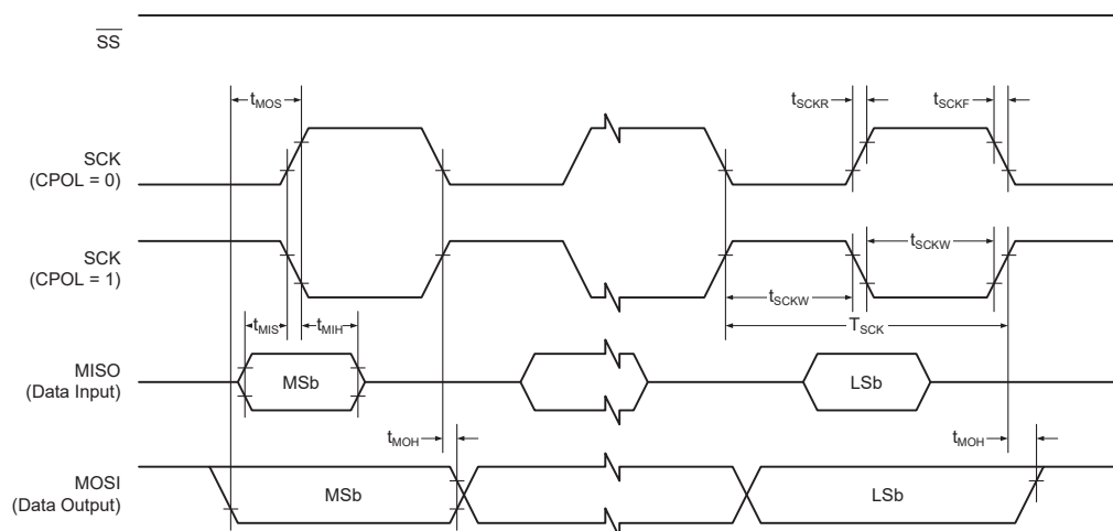
Figure 35-4. SPI - Timing Requirements in Host Mode
