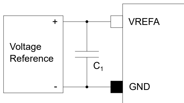
Figure 4-7. Recommended External Voltage Reference Connection
