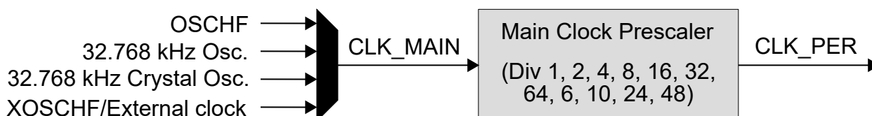
Figure 12-2. Main Clock and Prescaler
