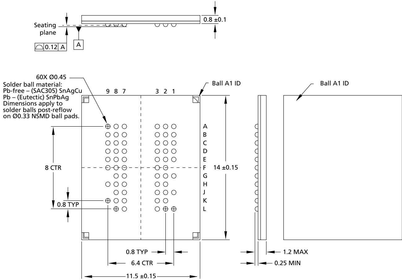
Figure 9: 60-Ball FBGA Package (11.5mm x 14mm) – x4, x8
