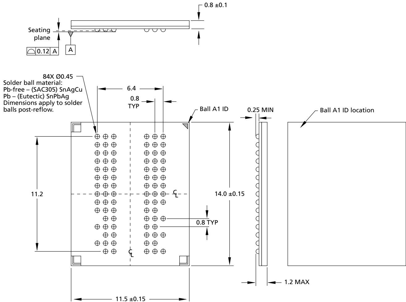
Figure 8: 84-Ball FBGA Package (11.5mm x 14mm) – x16
