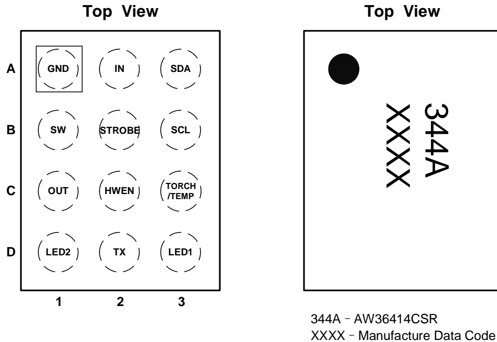
Fig 2 Pin Configuration and Top Mark
