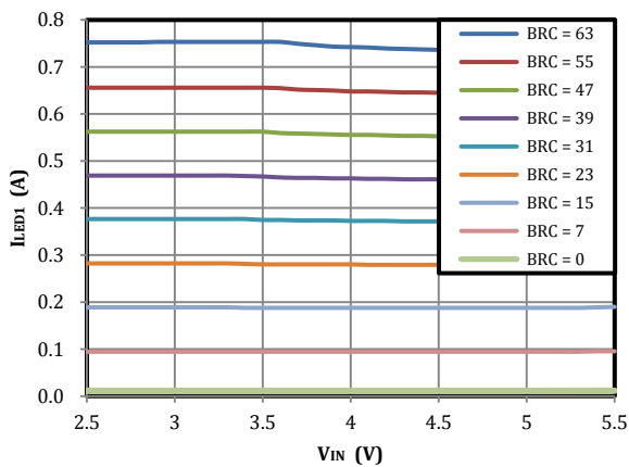
Fig 9. LED1 Flash Current vs Input Voltage
