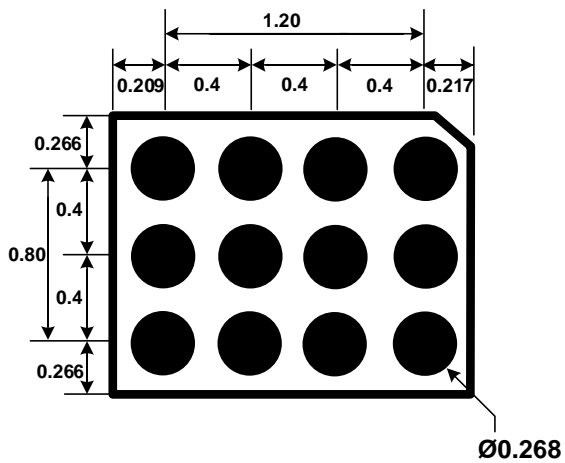
LAND PATTERN
