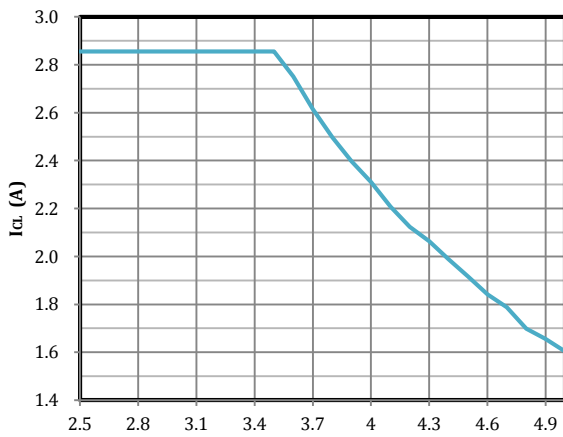
I LED =1.5A V IN (V) V LED =4.5V f sw =2MHz I CL =2.8A Inductor Current Limit vs Input Voltage
