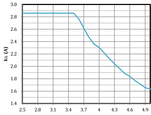
I LED =1.5A V IN (V) V LED =4.5V f sw =4MHz I CL =2.8A Inductor Current Limit vs Input Voltage
