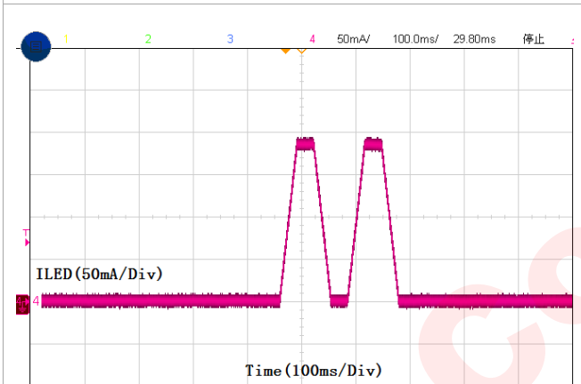
ILED=187.5mA breath twice(Reg0E(7:4)=0010)
