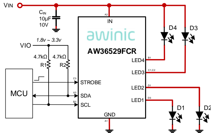
Fig 3 AW36529 Application Circuit
