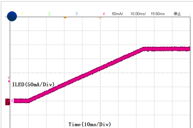
ILED=187.5mA Torch Ramp up=64ms(Reg0B(7:4)=0011)
