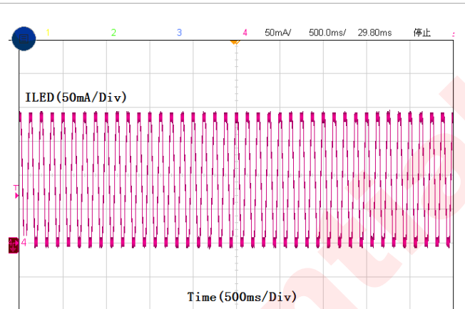
ILED=187.5mA Continuous breathing(Reg0E(7:4)=0000)
