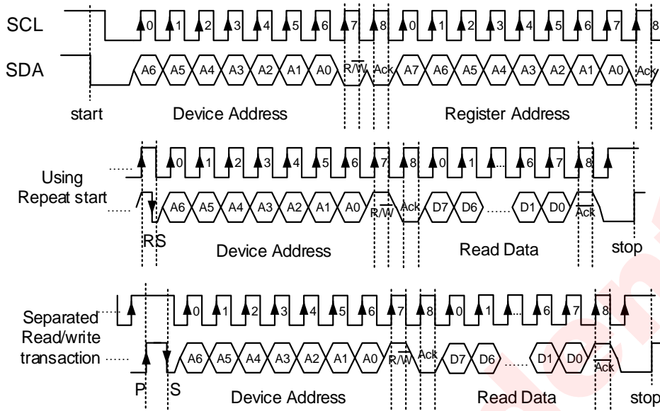
Fig 38 I 2 C Read Timing
