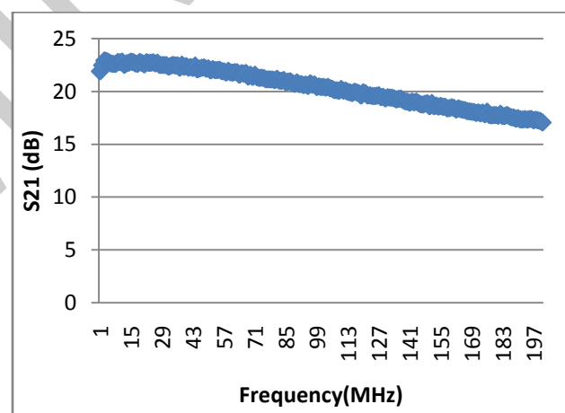
Figure 4 Power Gain(S21)
