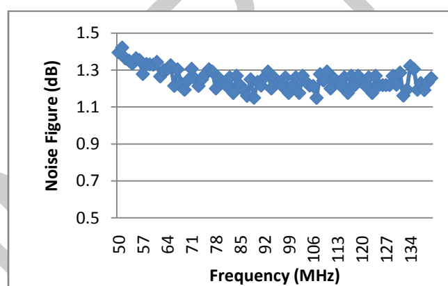
Figure 10 Noise Figure(NF)
