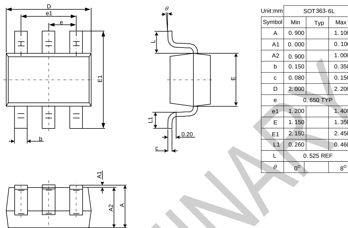
Figure 16 Package outline
