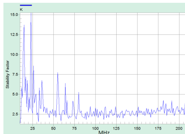
Figure 8 Stability Factor Kf
