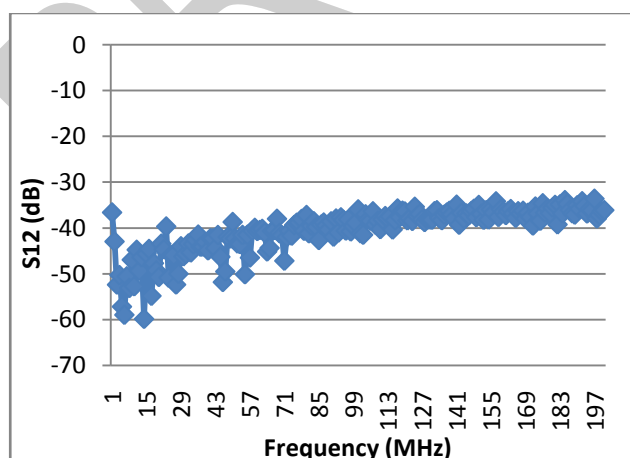
Figure 5 Reverse Isolation(S12)
