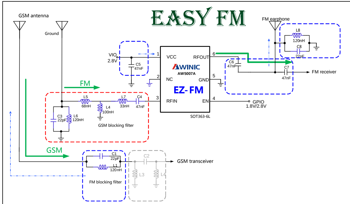
Figure 2 AW5007A typical application circuit
