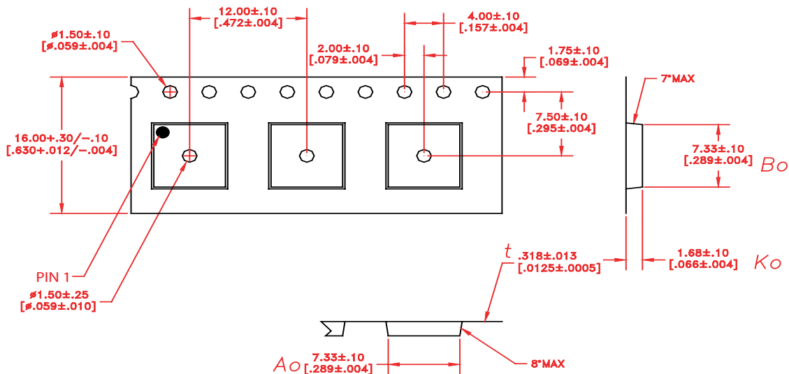
Figure 7: Tape &amp; Reel Packaging
