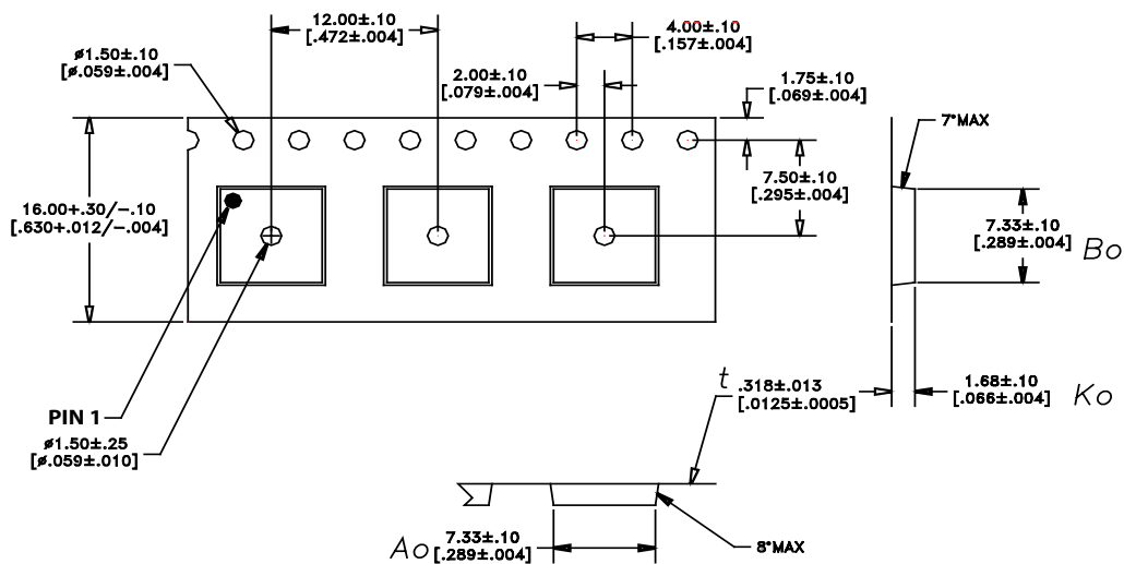
Figure 7: Tape &amp; Reel Packaging
