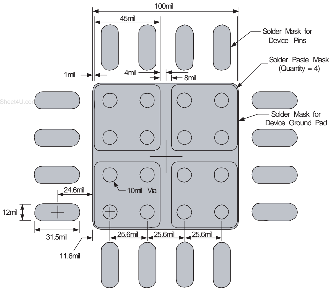
Figure 36: Recommended PCB Layout
