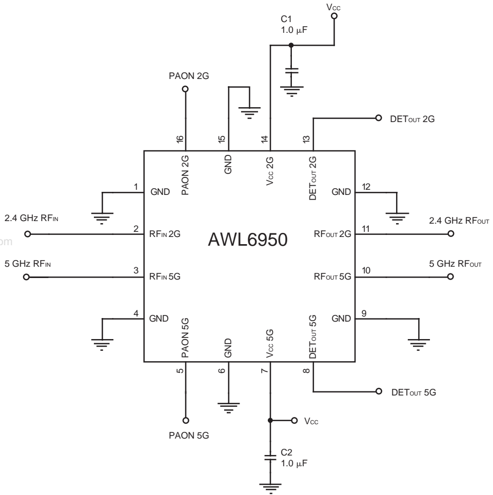
Figure 33: Application Circuit
