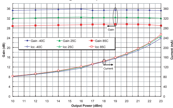
Figure 4: Gain and I_{CC} vs. Output Power Across Temp (Frequency = 2.45 GHz, V_{CC} = +3.3\text{ V} ) 802.11g 54 Mbps OFDM
