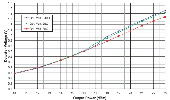
Figure 32: Detector Voltage vs. Output Power Across Temperature (Frequency = 2.45 GHz, V CC = +4.2 V) 802.11g 54 Mbps OFDM
