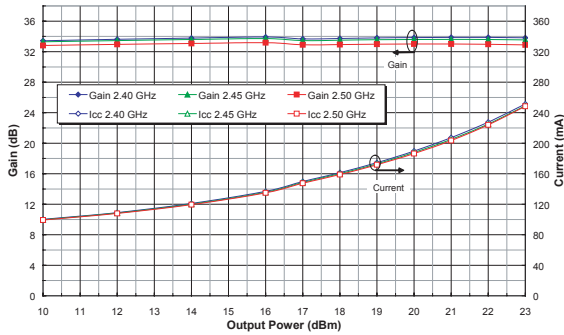
Figure 27: Gain and I CC vs. Output Power Across Frequency (V CC = +4.2 V, T C = +25°C) 802.11g 54 Mbps OFDM
