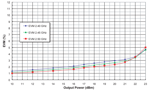
Figure 28: EVM vs. Output Power Across Frequency (V CC = +4.2 V, T C = 25°C) 802.11g 54 Mbps OFDM
