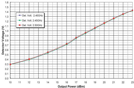
Figure 31: Detector Voltage vs. Output Power Across Frequency (T C = 25°C, V CC = +4.2 V) 802.11g 54 Mbps OFDM
