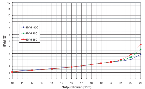
Figure 30: EVM vs. Output Power Across Temp (Frequency = 2.45 GHz, V CC = +4.2 V) 802.11g 54 Mbps OFDM
