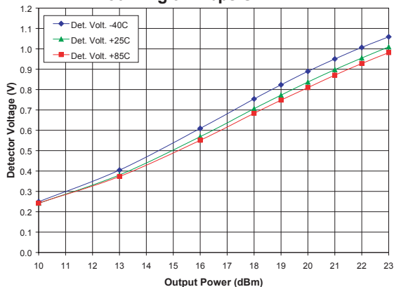
Figure 9: Detector Voltage vs. Output Power Across Temp. (Freq = 2.45 GHz, V_{CC} = +3.3\text{V} ) 802.11g 54 Mbps OFDM
