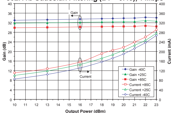
Figure 11: Gain and I_{CC} vs. Output Power Across Temp. (Frequency = 2.45GHz, V_{CC} = +3.3\text{V} ) 802.11b Gaussian Filtering (BT = 0.45), 1 Mbps
