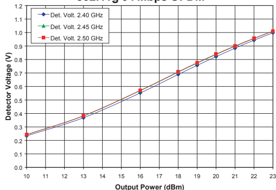
Figure 8: Detector Voltage vs. Output Power Across Frequency ( T_c = 25^\circ\text{C} , V_{CC} = +3.3\text{V} ) 802.11g 54 Mbps OFDM
