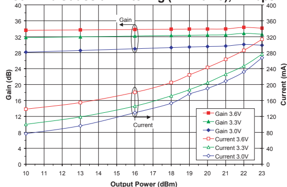
Figure 12: Gain and I_{CC} vs. Output Power Across Power Supply Voltage (Freq = 2.45GHz, T_c = 25^\circ\text{C} ) 802.11b Gaussian Filtering (BT = 0.45), 1 Mbps
