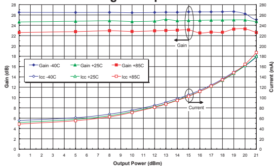
Figure 3: Tx Path Gain and Icc vs. Output Power Across Temp (Freq = 2.45 GHz, V_{CC} = +3.8\text{ V} ) 802.11g 54 Mbps OFDM
