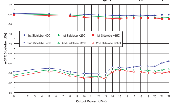
Figure 12: Tx Path ACPR Sidelobes 1&2 vs. Output Power Across Temp (Freq = 2.45 GHz, V_{CC} = +3.8 V) 802.11b Root Cosine Filtering (bT = 0.5), 1 Mbps
