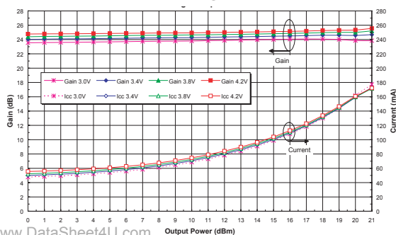
Figure 4: Tx Path Gain and Icc vs. Output Power Across Supply Voltage (Freq = 2.45 GHz, T_A = +25^\circ\text{C} ) 802.11g 54 Mbps OFDM
