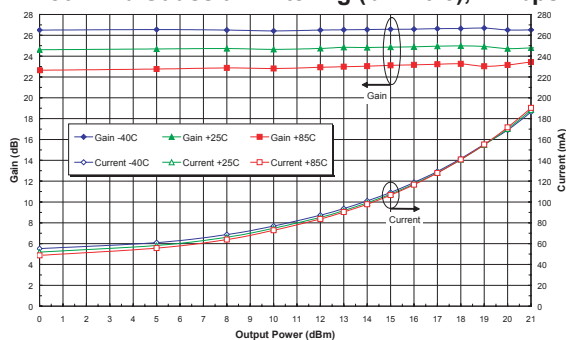
Figure 9: Tx Path Gain and Icc vs. Output Power Across Temp (Freq = 2.45 GHz, V_{CC} = +3.8 V) 802.11b Gaussian Filtering (bT = 0.5), 1 Mbps
