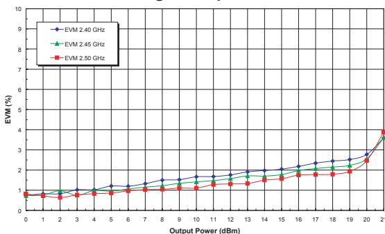
Figure 5: Tx Path EVM vs. Output Power Across Frequency ( V_{CC} = +3.8\text{ V} , T_A = +25^\circ\text{C} ) 802.11g 54 Mbps OFDM
