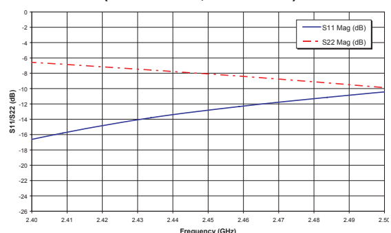
Figure 17: 2.4 GHz Tx Path S-Parameters S11 & S22 Response (Narrow band) (V CC = +3.8 V, T A = +25°C)
