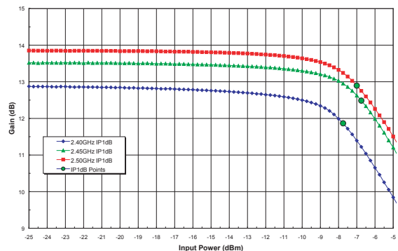
Figure 19: Receive Path Input P1dB Across Freq (V CC = +3.8, V LNA_EN = +3.1 V, T = +25°C)
