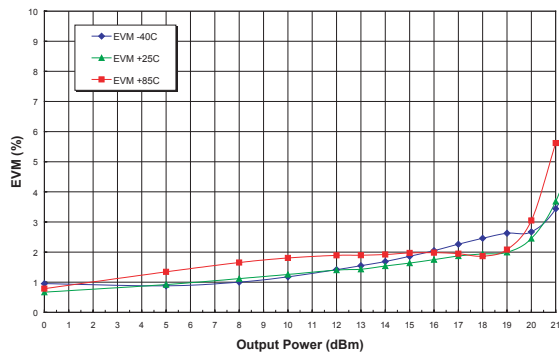
Figure 6: Tx Path EVM vs. Output Power Across Temp (Freq = 2.45 GHz, V_{CC} = +3.8\text{ V} ) 802.11g 54 Mbps OFDM
