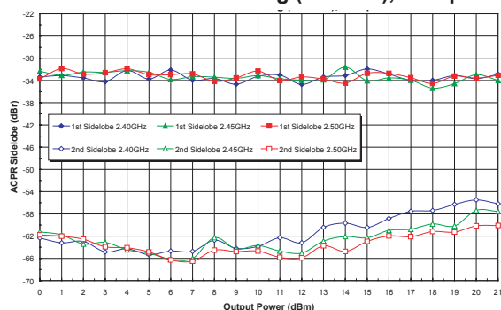
Figure 11: Tx Path ACPR Sidelobes 1&2 vs. Output Power Across Freq ( V_{CC} = +3.8 V, T_A = +25^\circ\text{C} ) 802.11b Gaussian Filtering (bT = 0.5), 1 Mbps
