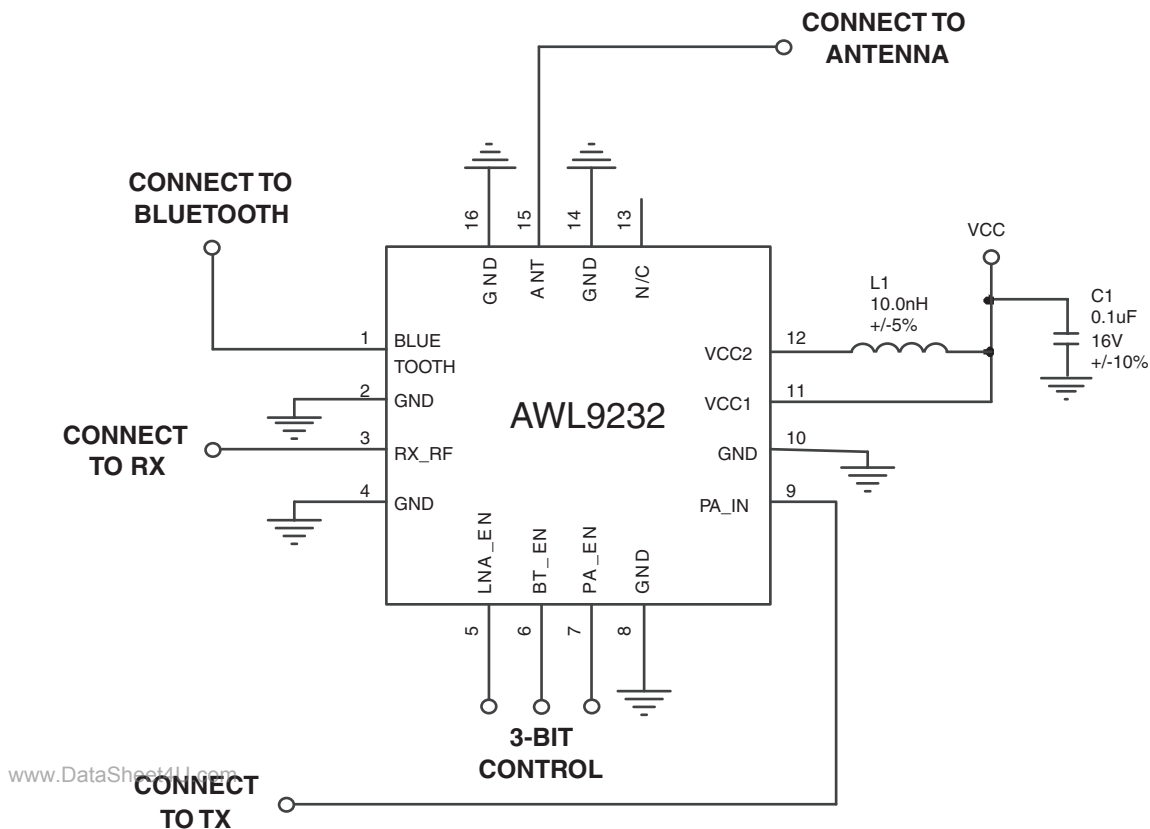
Figure 26: Application Circuit
