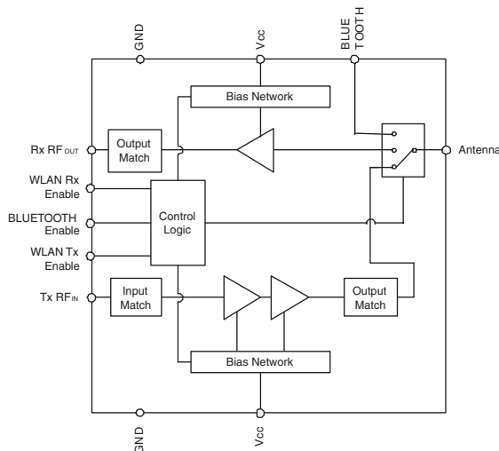
Figure 1: Block Diagram and Pinout
