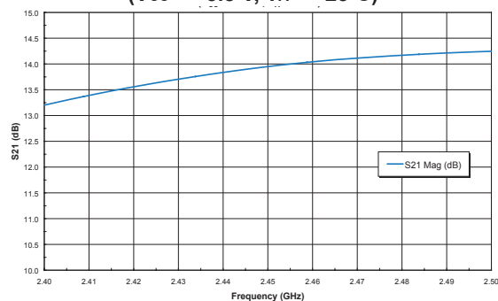
Figure 22: Rx Path S-Parameters S21 Response (Narrow band) ( V_{CC} = +3.8\text{ V} , T_A = +25^\circ\text{C} )
