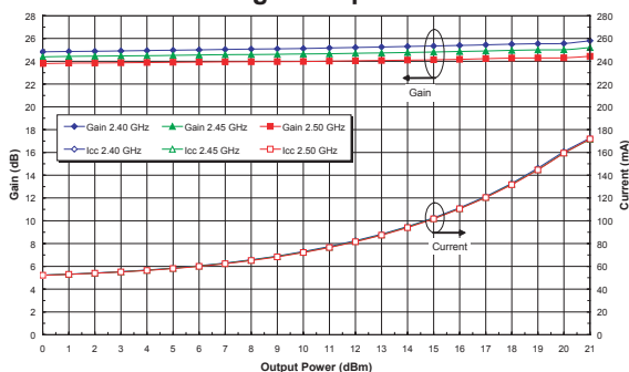
Figure 2: Tx Path Gain and Icc vs. Output Power Across Freq ( V_{CC} = +3.8\text{ V} , T_A = +25^\circ\text{C} ) 802.11g 54 Mbps OFDM
