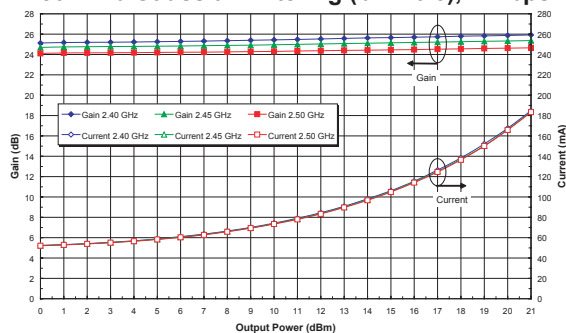
Figure 8: Tx Path Gain and Icc vs. Output Power Across Freq ( V_{CC} = +3.8 V, T_A = +25^\circ\text{C} ) 802.11b Gaussian Filtering (bT = 0.5), 1 Mbps
