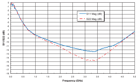
Figure 25: Bluetooth S-Parameters S11 & S22 Response ( V_{CC} = +3.8\text{ V} , T_A = +25^\circ\text{C} )
