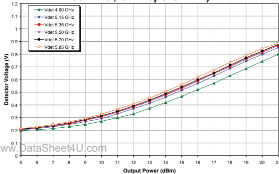
Figure 29: Voltage Detector vs. Output Power Across Frequency (Vcc = +3.3 V, Temp = -40 °C 802.11a, 54 Mbps OFDM)
