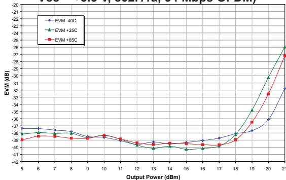
Figure 19: Tx Path Dynamic EVM vs. Output Power Across Temperature (Freq = 5.5 GHz, Vcc = +3.3 V, 802.11a, 54 Mbps OFDM)
