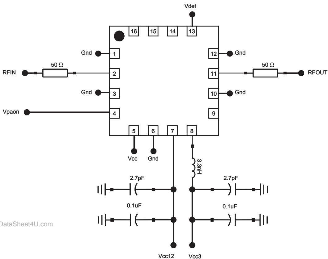
Figure 33: Application Circuit
