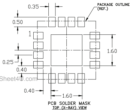
Figure 35: Recommended PCB Layout
