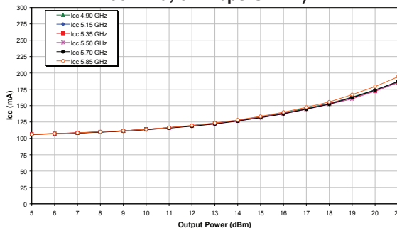
Figure 13: Tx Path Icc vs. Output Power Across Frequency (Vcc = +3.0 V, Temp = +25 °C 802.11a, 54 Mbps OFDM)
