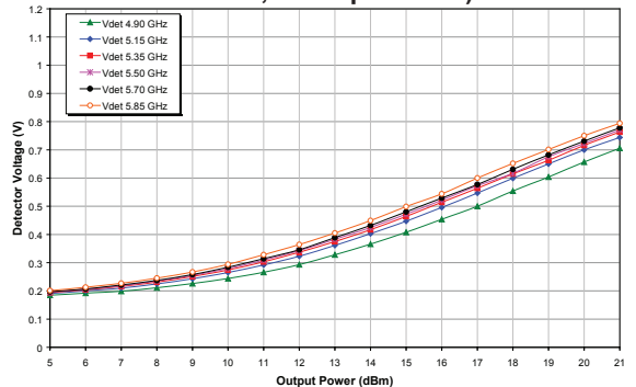
Figure 30: Voltage Detector vs. Output Power Across Frequency (Vcc = +3.3 V, Temp = +85 °C 802.11a, 54 Mbps OFDM)
