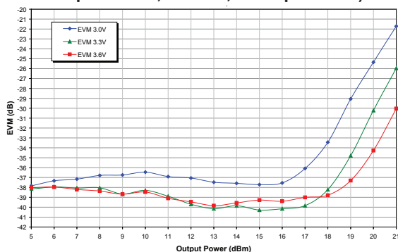
Figure 18: Tx Path Dynamic EVM vs. Output Power Across Voltage (Freq = 5.5 GHz, Temp = +25 °C, 802.11a, 54 Mbps OFDM)
