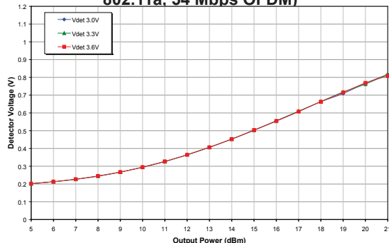
Figure 25: Voltage Detector vs. Output Power Across Voltage (Freq = 5.5 GHz, Temp = +25\text{ }^{\circ}\text{C} , 802.11a, 54 Mbps OFDM)
