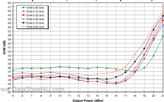
Figure 23: Tx Path Dynamic EVM vs. Output Power Across Frequency ( V_{cc} = +3.3\text{ V} , Temp = +85\text{ }^{\circ}\text{C} , 802.11a, 54 Mbps OFDM)
