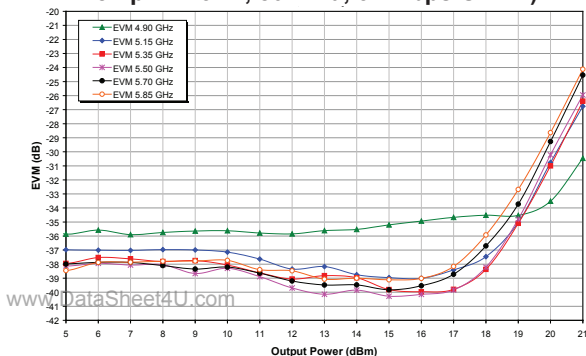
Figure 17: Tx Path Dynamic EVM vs. Output Power Across Frequency (Vcc = +3.3V, Temp = +25 °C, 802.11a, 54 Mbps OFDM)
