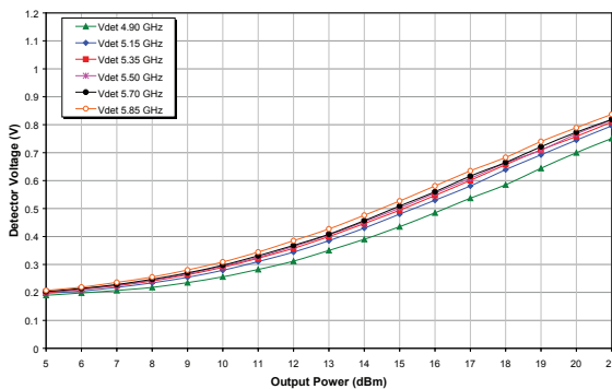
Figure 27: Voltage Detector vs. Output Power Across Frequency (Vcc = +3.0 V, Temp = +25 °C 802.11a, 54 Mbps OFDM)
