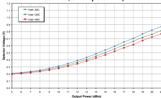
Figure 26: Voltage Detector vs. Output Power Across Temperature (Freq = 5.5 GHz, V_{cc} = +3.3\text{ V} , 802.11a, 54 Mbps OFDM)
