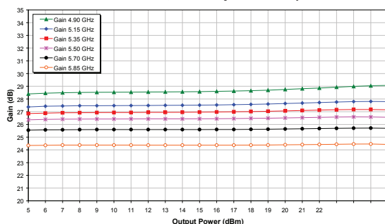
Figure 9: Tx Path Gain vs. Output Power Across Frequency (Vcc = +3.3 V, Temp = +85 °C 802.11a, 54 Mbps OFDM)
