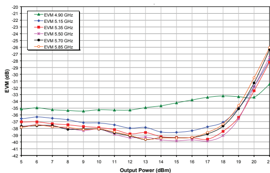
Figure 22: Tx Path Dynamic EVM vs. Output Power Across Frequency ( V_{cc} = +3.3\text{ V} , Temp = -40\text{ }^{\circ}\text{C} , 802.11a, 54 Mbps OFDM)
