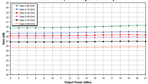
Figure 6: Tx Path Gain vs. Output Power Across Frequency ( V_{cc} = +3.0 V , Temp = +25 °C 802.11a, 54 Mbps OFDM)
