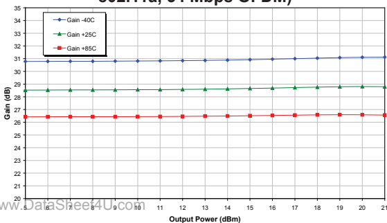
Figure 5: Tx Path Gain vs. Output Power Across Temperature (Freq = 5.5 GHz, V_{cc} = +3.3 V 802.11a, 54 Mbps OFDM)
