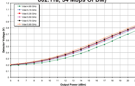
Figure 24: Voltage Detector vs. Output Power Across Frequency ( V_{cc} = +3.3\text{ V} , Temp = +25\text{ }^{\circ}\text{C} , 802.11a, 54 Mbps OFDM)
