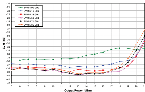
Figure 21: Tx Path Dynamic EVM vs. Output Power Across Frequency ( V_{cc} = +3.6\text{ V} , Temp = +25\text{ }^{\circ}\text{C} , 802.11a, 54 Mbps OFDM)
