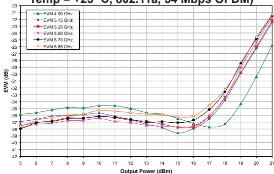
Figure 20: Tx Path Dynamic EVM vs. Output Power Across Frequency (Vcc = +3.0 V, Temp = +25 °C, 802.11a, 54 Mbps OFDM)
