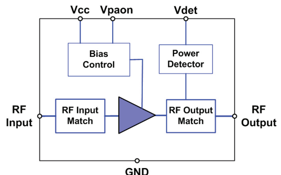
Figure 1: Block Diagram and Pinout
