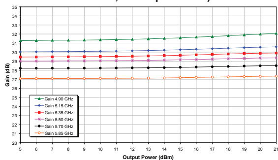
Figure 7: Tx Path Gain vs. Output Power Across Frequency ( V_{cc} = +3.6 V , Temp = +25 °C 802.11a, 54 Mbps OFDM)
