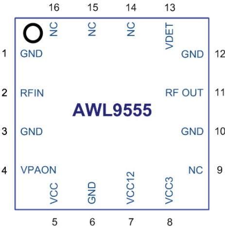
Figure 2: Pinout Diagram (Top View)
