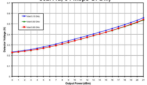
Figure 12: Voltage Detector vs. Output Power Across Frequency ( V_{CC} = +3.3 V, Temp = 25 °C, 802.11a, 54 Mbps OFDM)
