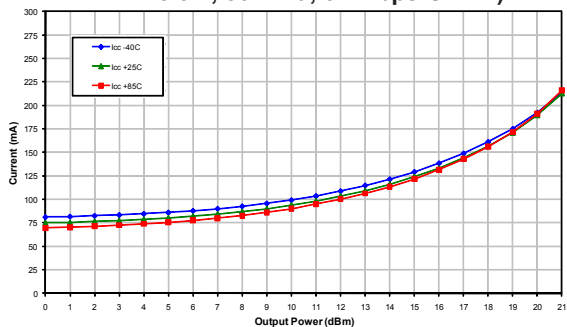
Figure 8: Tx Path I_{CC} vs. Output Power Across Temperature (Freq = 5.5 GHz, V_{CC} = +3.3 V, 802.11a, 54 Mbps OFDM)
