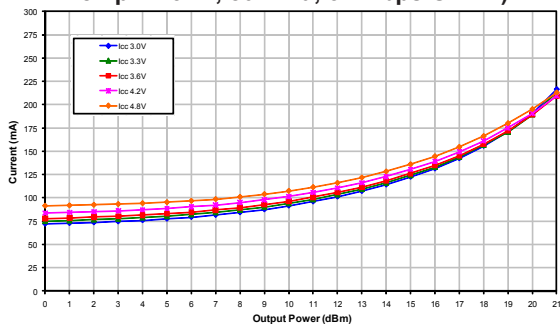
Figure 7: Tx Path I_{CC} vs. Output Power Across Voltage (Freq = 5.5 GHz, Temp = 25 °C, 802.11a, 54 Mbps OFDM)
