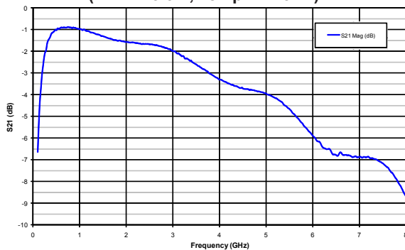
Figure 21: 2 GHz Tx Path Response ( V_{CC} = +3.3 V, Temp = +25 °C)
