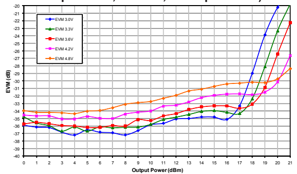
Figure 10: Tx Path Dynamic EVM vs. Output Power Across Voltage (Freq = 5.5 GHz, Temp = 25 °C, 802.11a, 54 Mbps OFDM)
