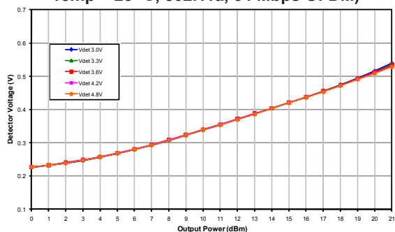
Figure 13: Voltage Detector vs. Output Power Across Voltage (Freq = 5.5 GHz, Temp = 25 °C, 802.11a, 54 Mbps OFDM)
