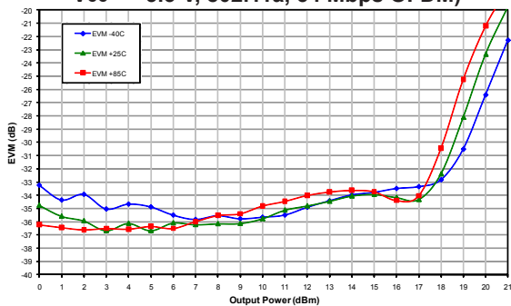
Figure 11: Tx Path Dynamic EVM vs. Output Power Across Temperature (Freq = 5.5 GHz, V_{CC} = +3.3 V, 802.11a, 54 Mbps OFDM)
