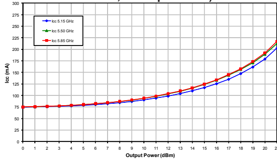
Figure 6: Tx Path I_{CC} vs. Output Power Across Frequency ( V_{CC} = +3.3 V, Temp = 25 °C, 802.11a, 54 Mbps OFDM)
