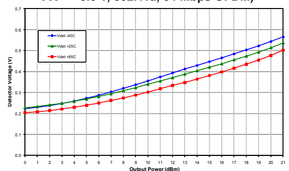
Figure 14: Voltage Detector vs. Output Power Across Temperature (Freq = 5.5 GHz, V_{CC} = +3.3 V, 802.11a, 54 Mbps OFDM)
