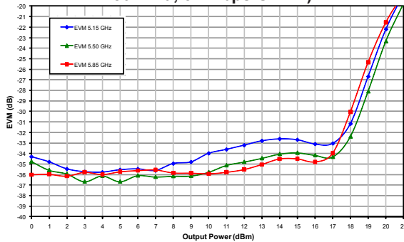
Figure 9: Tx Path Dynamic EVM vs. Output Power Across Frequency ( V_{CC} = +3.3 V, Temp = 25 °C, 802.11a, 54 Mbps OFDM)
