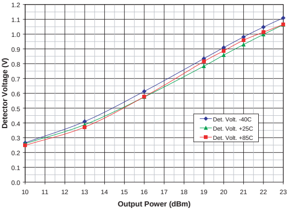
Figure 9: Detector Voltage vs. Output Power Across Temp. (Freq = 2.45 GHz, V_{CC} = +3.3\text{ V} , 2\text{ K}\Omega Load) 2.4 GHz 802.11g 54 Mbps OFDM
