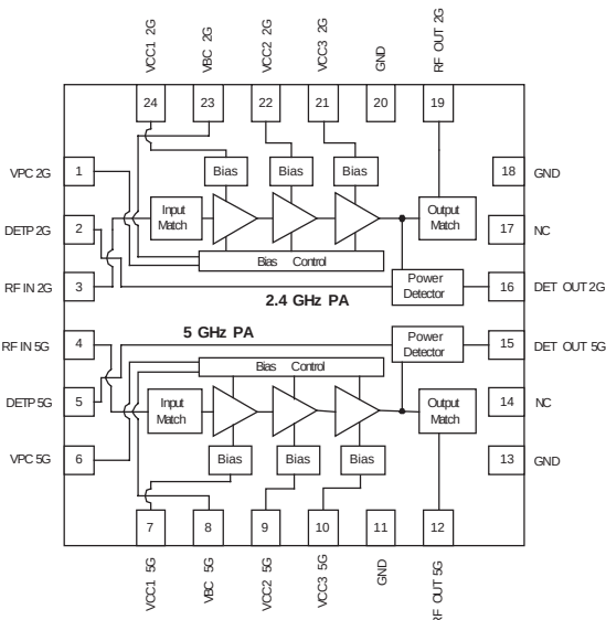
Figure 1: Block Diagram and Pinout www.DataSheet4U.com
