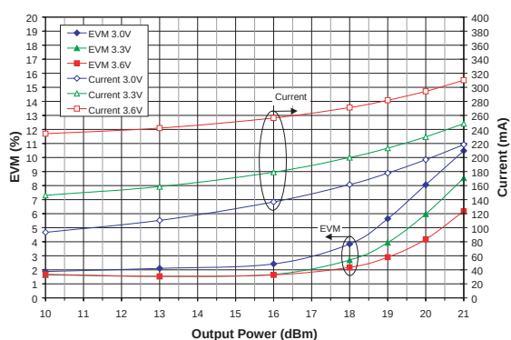
Figure 25: I_{CC} and EVM vs. Output Power Across Supply Voltage (\text{Freq} = 5.40 \text{ GHz}, T_c = 25^\circ\text{C}) 5 GHz 802.11a 54 Mbps OFDM
