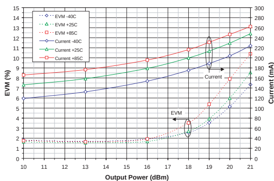
Figure 23: I_{CC} and EVM vs. Output Power Across Temp (\text{Freq} = 5.4 \text{ GHz}, V_{CC} = +3.3 \text{ V}) 5 GHz 802.11a 54 Mbps OFDM
