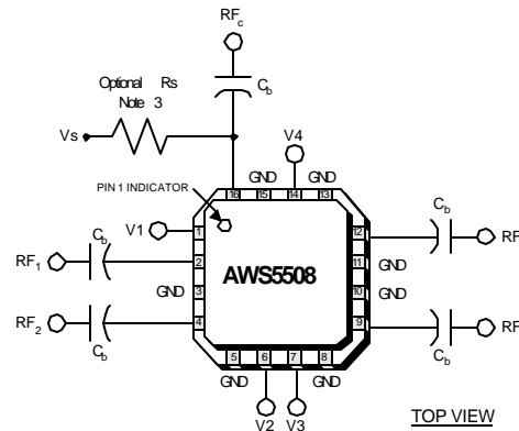
Figure 1: Pin Out Diagram
