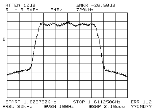
Figure 3: ACPR @ P_{OUT} = 35 dBm
