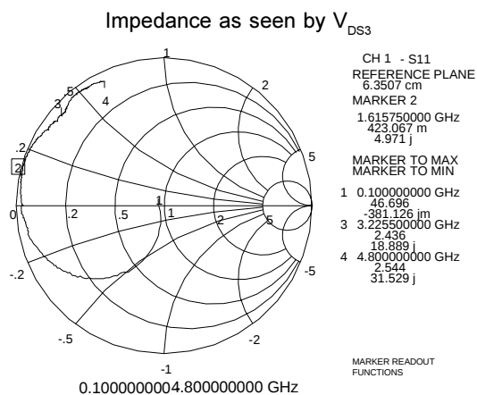
Figure 8: S11 Forward Reflection Impedance
