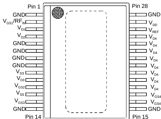
Figure 1: Pin Layout
