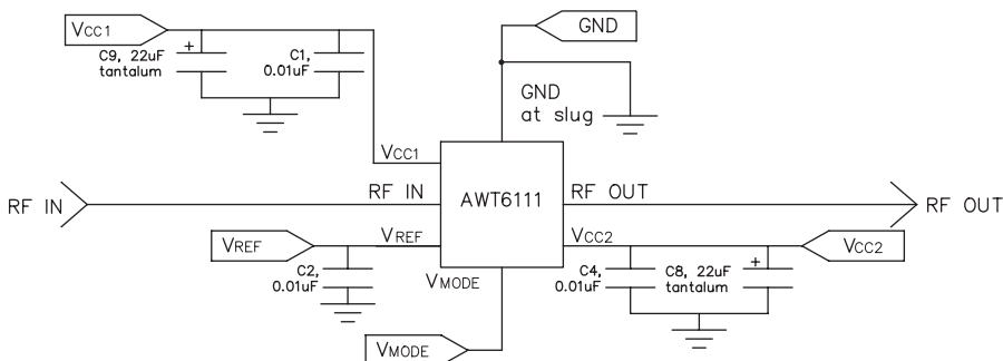
Figure 1: Application Schematic
