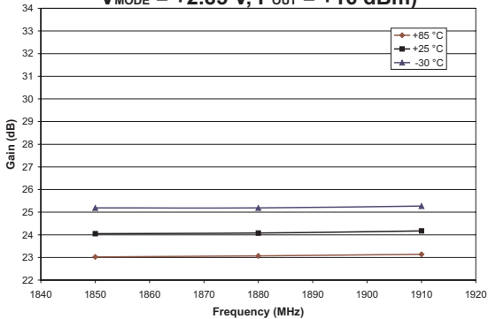
Figure 8: Large Signal Gain vs. Frequency +3.2 V Supply, Low Bias Mode (T C = +25 °C, V CC = +3.2 V, V REF = +2.85 V, V MODE = +2.85 V, P OUT = +16 dBm)
