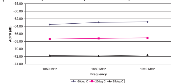
Figure 8: ACP2 vs. Frequency P_{OUT} = +16 dBm, Low Bias Mode (T_C = +25 °C, V_{CC} = +3.4 V, V_{REF} = +2.9 V, V_{MODE} = +2.9 V)
