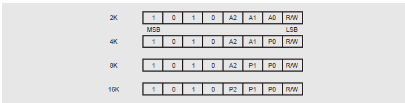
Figure 4: Device Address
