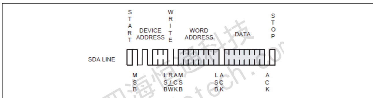
Figure 5: Byte Write
