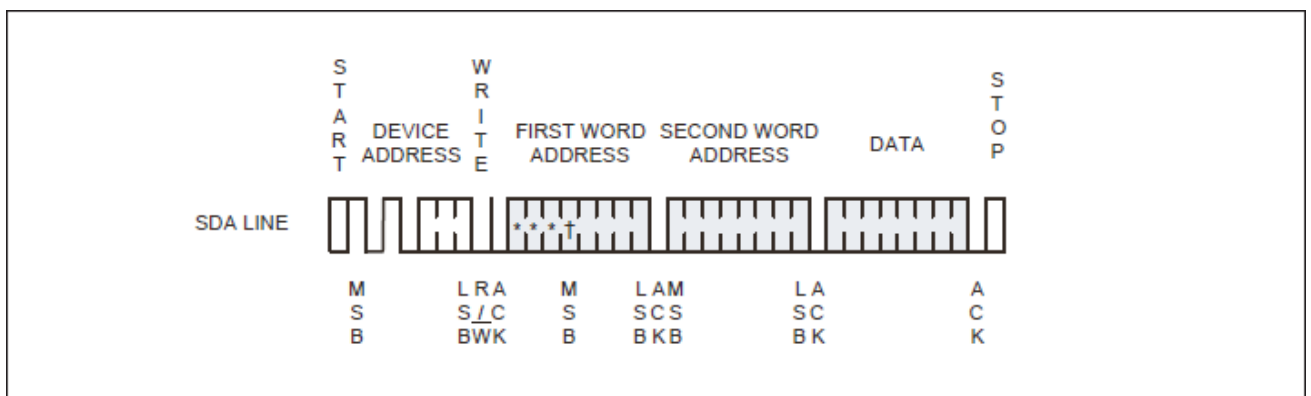
Figure 5: Byte Write
