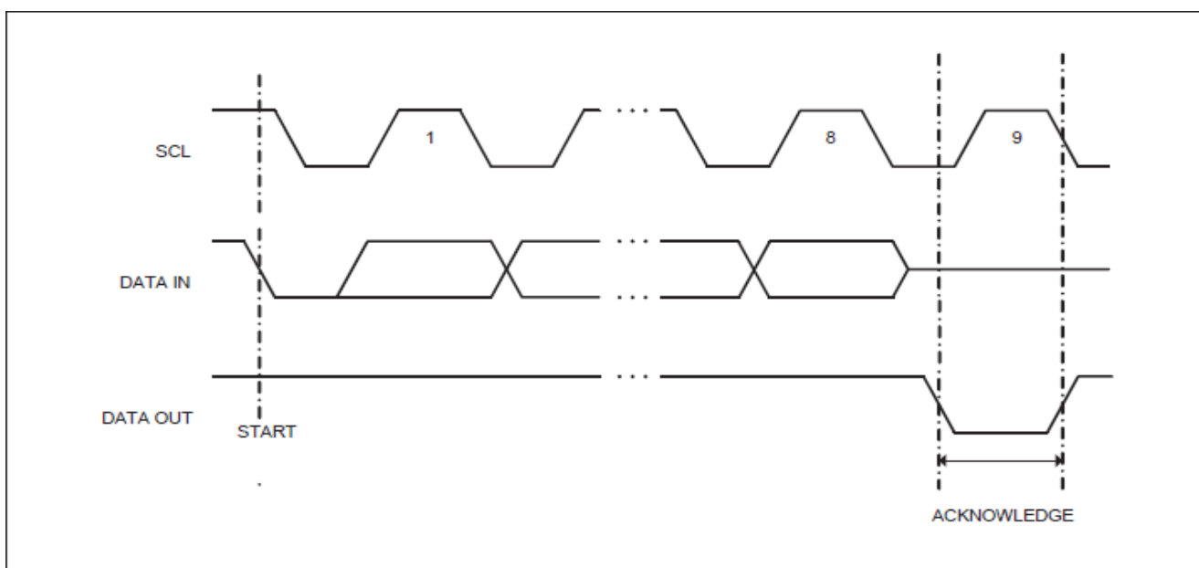
Figure 3: Output Acknowledge
