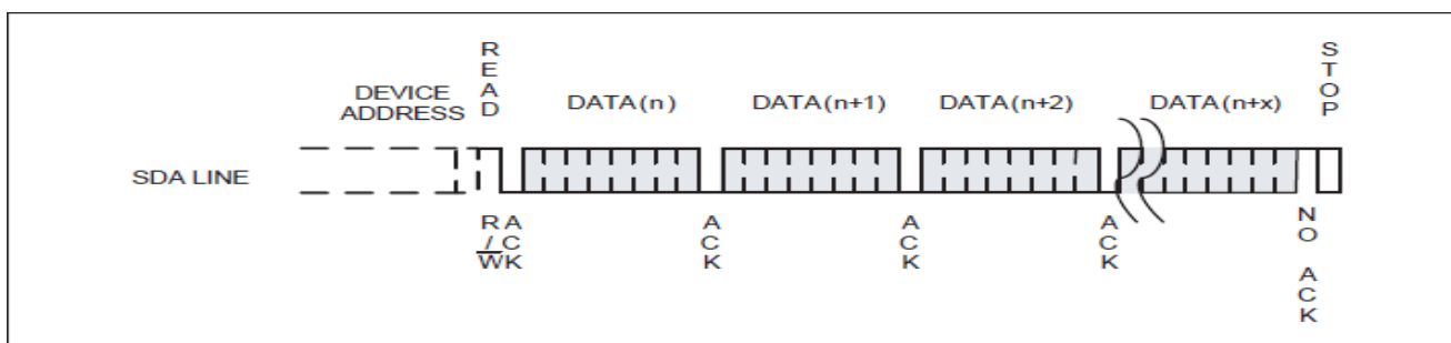
Figure 9: Sequential Read
