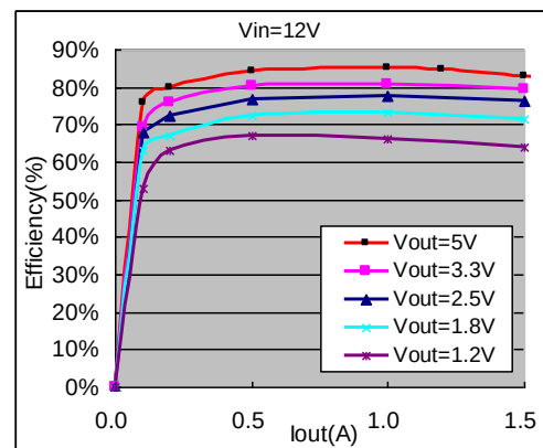
Efficiency ( V_{IN}=12V )
