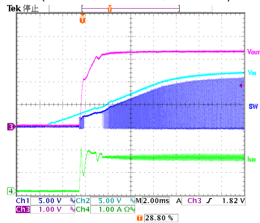
EN PIN on test wave ( V_{IN}=12V , V_{OUT}=3.3V , I_{OUT}=1.5A )
