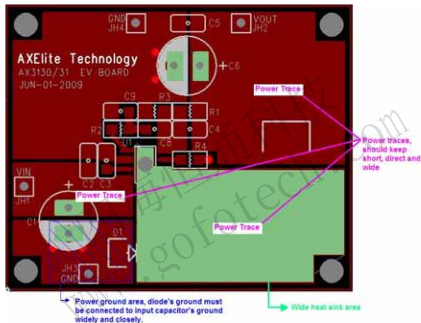
AX3130 PCB Layout – Top layer
