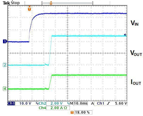
Enable-ON Wave (60KHz) ( V_{IN}=24V, V_{OUT}=5V, Load=2A, C_{EN/SS}=0.1\mu F )
