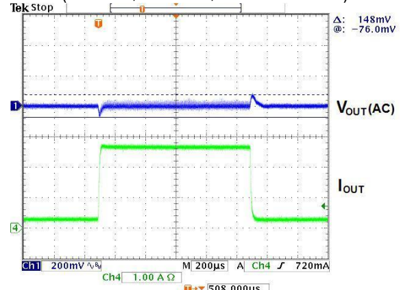
Load Transient (F=60KHz) ( V_{IN}=24V, V_{OUT}=5V, Load=0.3\sim 2.7A )
