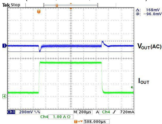
Load Transient (F=60KHz) ( V_{IN}=12V, V_{OUT}=5V, Load=0.3\sim 2.7A )
