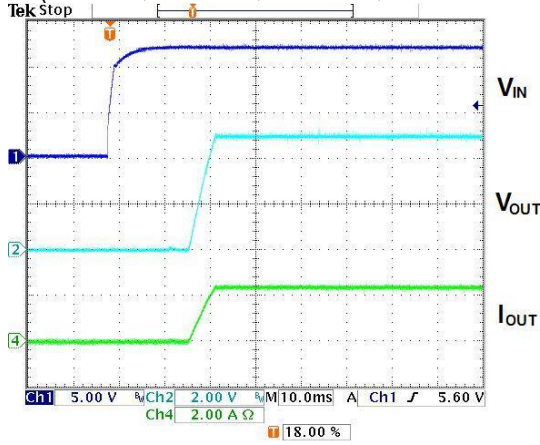
Enable-ON Wave (60KHz) ( V_{IN}=12V, V_{OUT}=5V, Load=2A, C_{EN/SS}=0.1\mu F )
