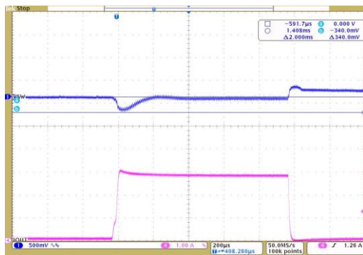
Load Transient
