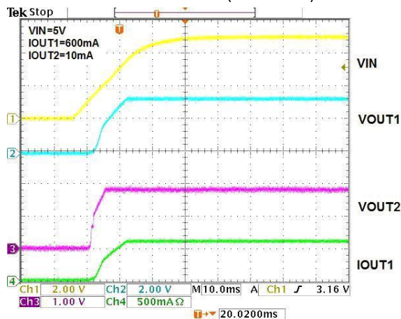
Enable -ON Test (Channel 1)
