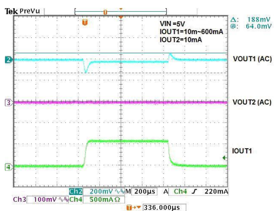
Load Transient (Channel 1)
