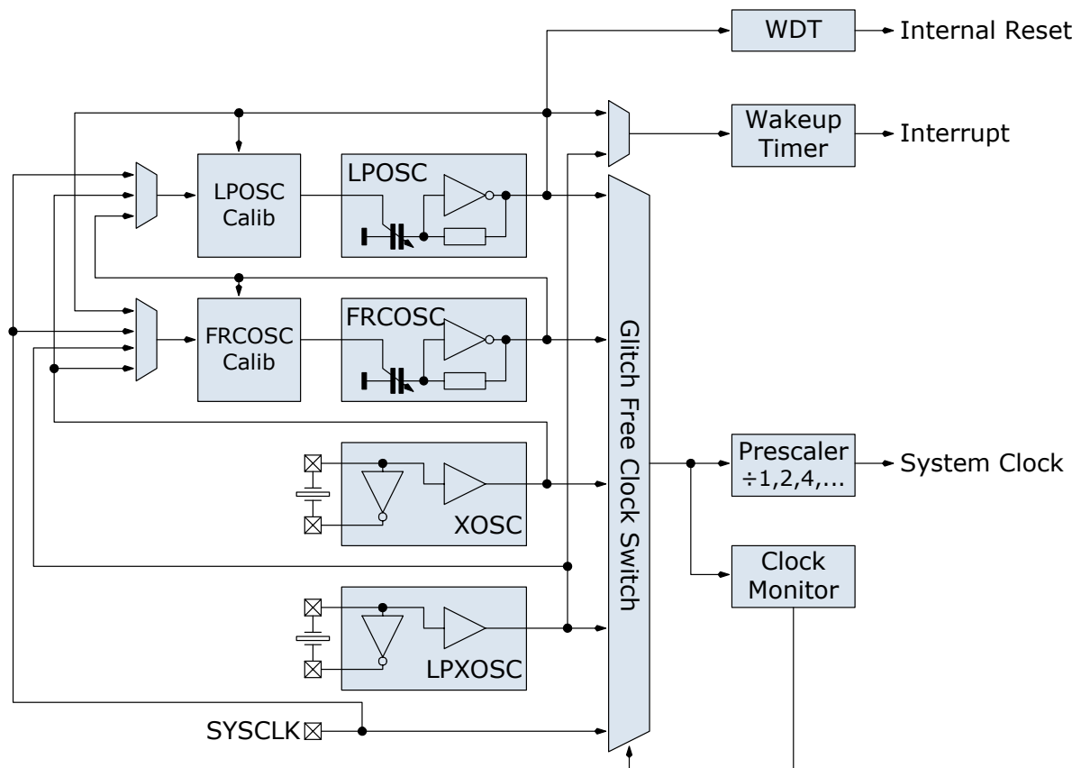
Figure 6 Clock System Diagram
