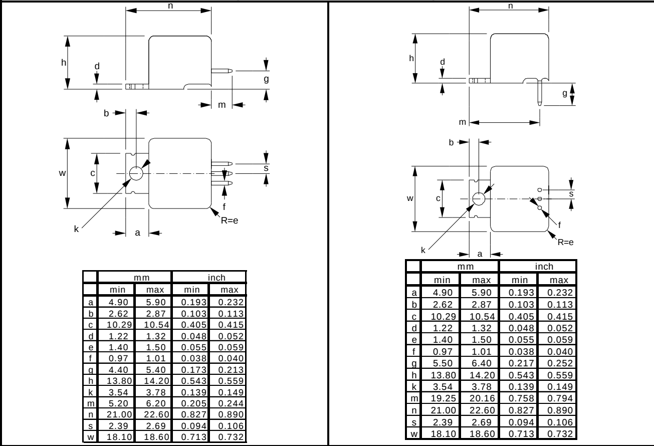
Fig6. - Mechanical Drawing
