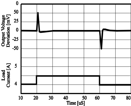
Fig5. - Load Transient Response
