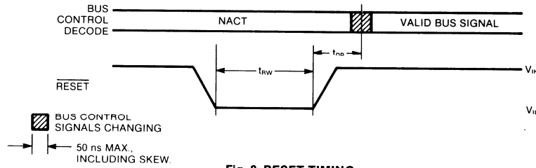
Fig. 8 RESET TIMING
