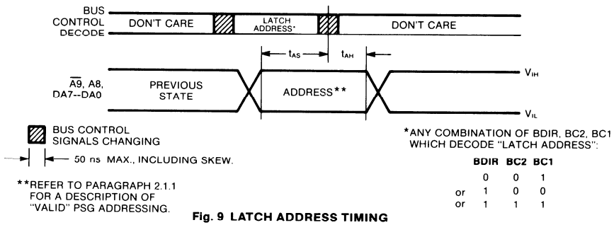
Fig. 9 LATCH ADDRESS TIMING
