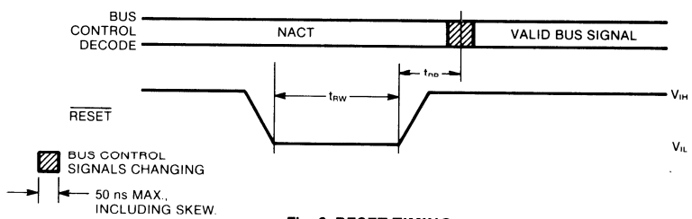
Fig. 8 RESET TIMING
