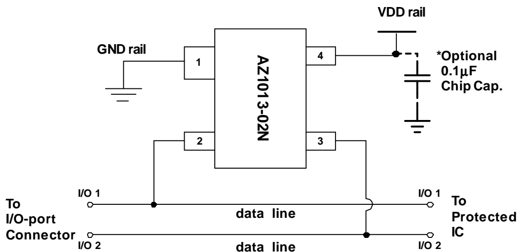
Fig. 2 Data lines and power rails connection of AZ1013-02N.
