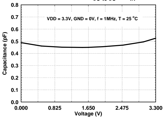
Typical Variation of C_{I/O\text{-to-I/O}} vs. V_{IN}
