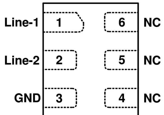
DFN1210P6X (Top View)
