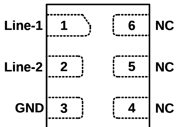
DFN1210P6X (Top View)
