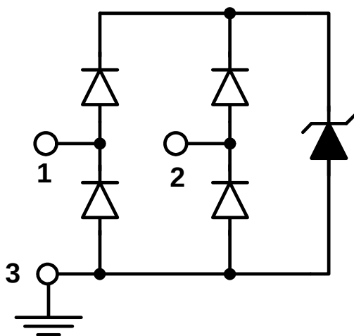
Circuit Diagram
