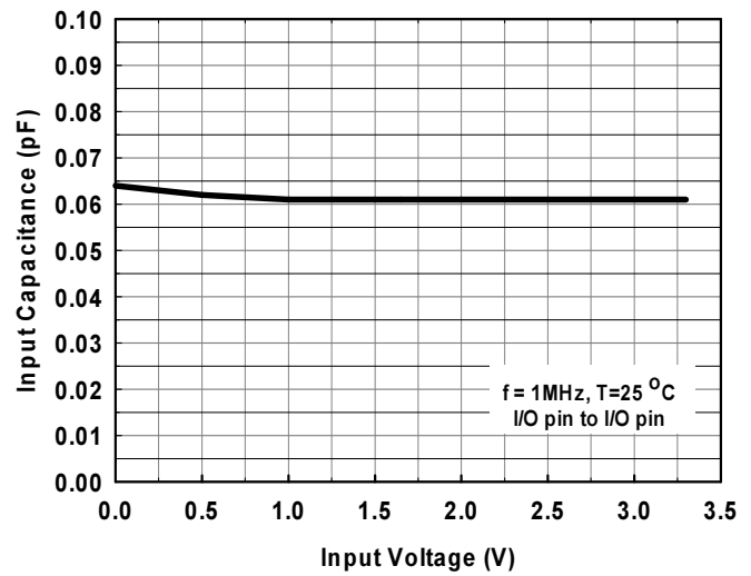
Typical variation of C_{IO\text{-to-}IO} vs. V_{IN}
