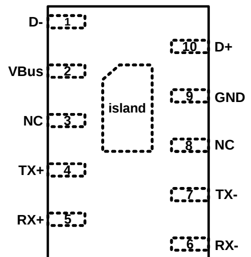
DFN4120P10E (Top View)
