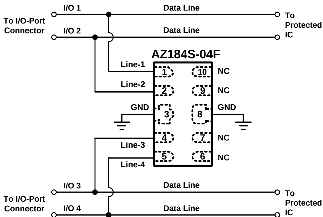
Fig. 1 Data lines connection of AZ184S-04F.
