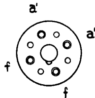
OCTAL BASE
