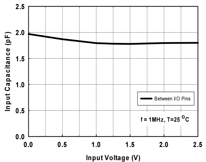
Typical Variation of C_{IN} vs. V_{IN}
