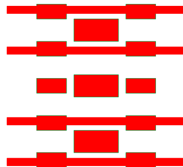
Fig. 2 Layout example of AZ3125-08F.
