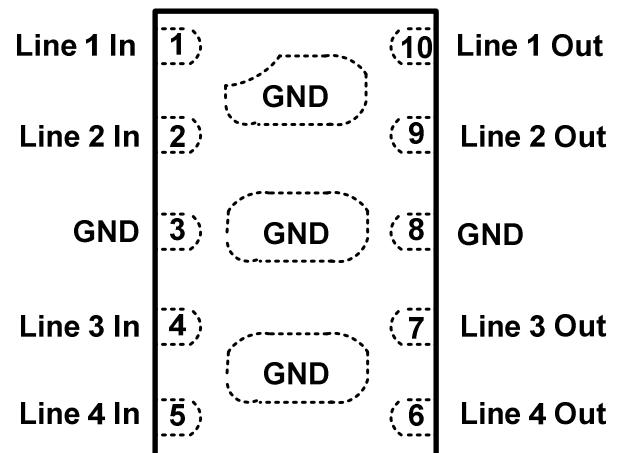
Fig. 1 Pin configuration of AZ3125-08F.
