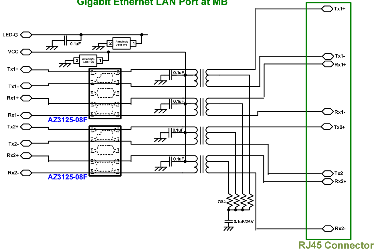
Fig. 3 Gigabit Ethernet surge protection circuit with AZ3125-08F.
