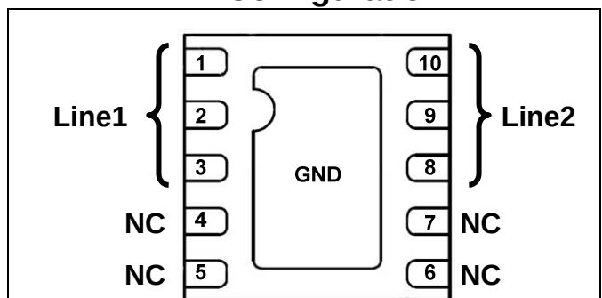
DFN2525P10E (2.5x2.5mm) (Top View)
