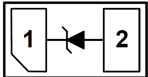
DFN1006P2X (Bottom View) (1.0mm x 0.6mm x 0.45mm)
