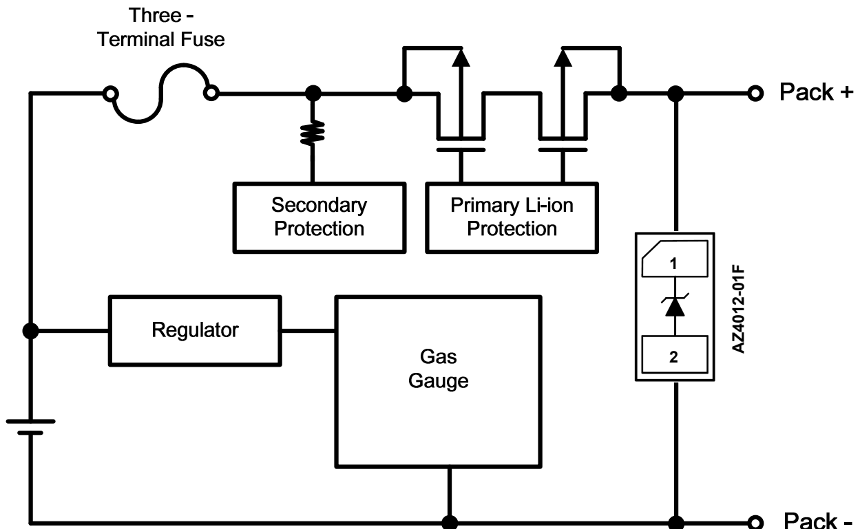
Fig. 1 ESD protection scheme for a typical Li-ion battery pack by using AZ4012-01F.
