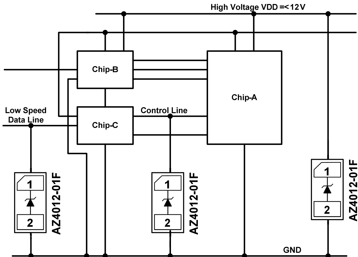
Fig. 2 ESD protection scheme for internal PCB circuits by using AZ4012-01F.
