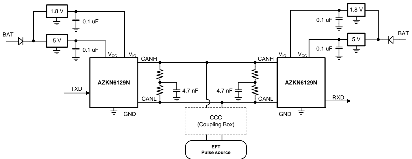
Figure 7. EFT coupling test circuit for AZKN6129N.
