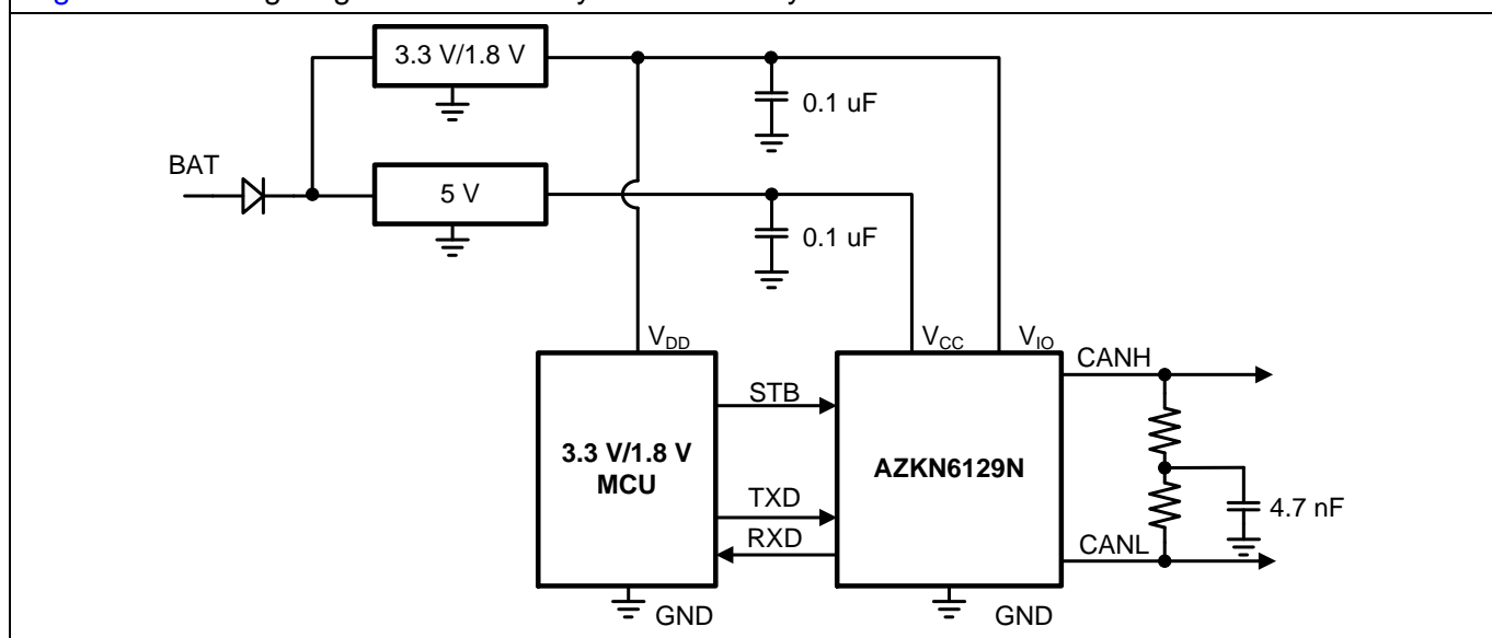
Figure 5. Typical application circuit for AZKN6129N with 3.3 V or 1.8 V MCU.
