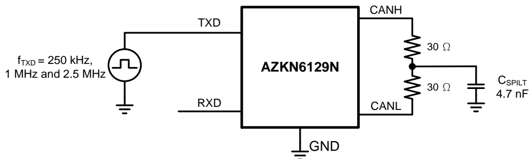
Figure 8. Test circuit for measuring transmitter driver symmetry.
