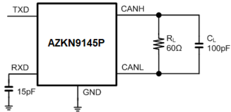
Figure 5. CAN transceiver timing test circuit.
