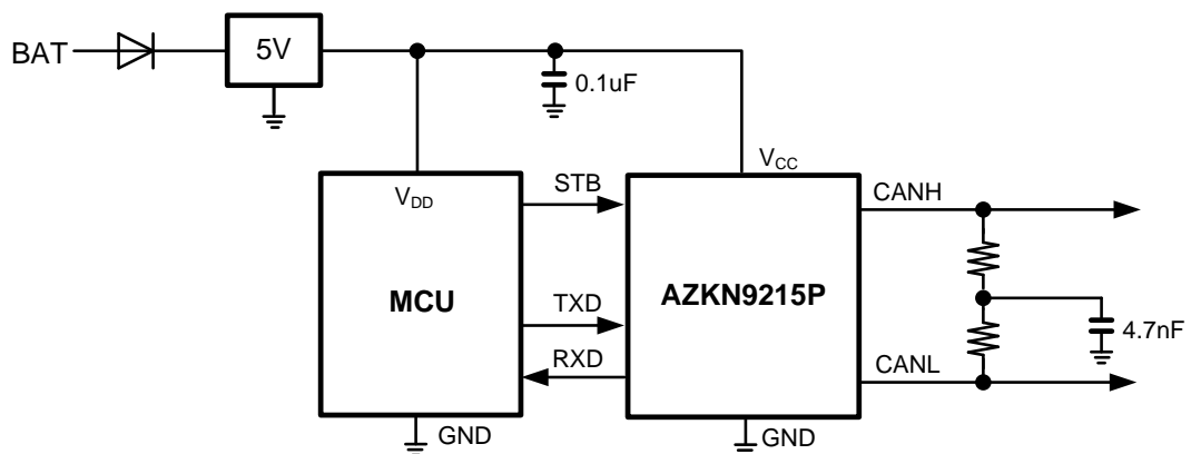
Figure 5. Typical application circuit for AZKN9215P with 5V MCU.
