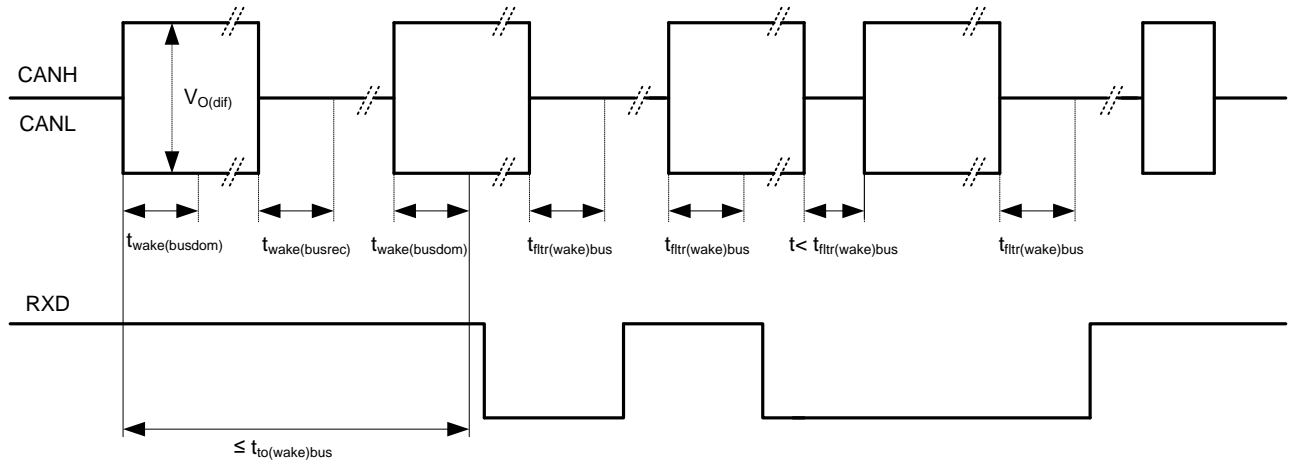
Figure 3. Timing diagram for wake-up pattern
