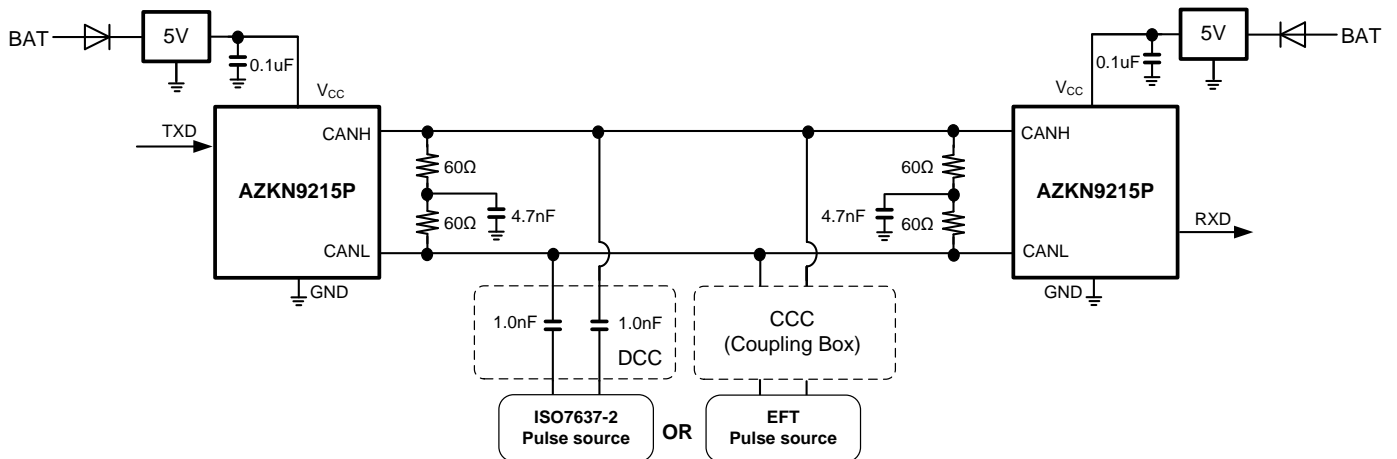
Figure 7. ISO 7637-2 DCC or EFT coupling test circuit for AZKN9215P.
