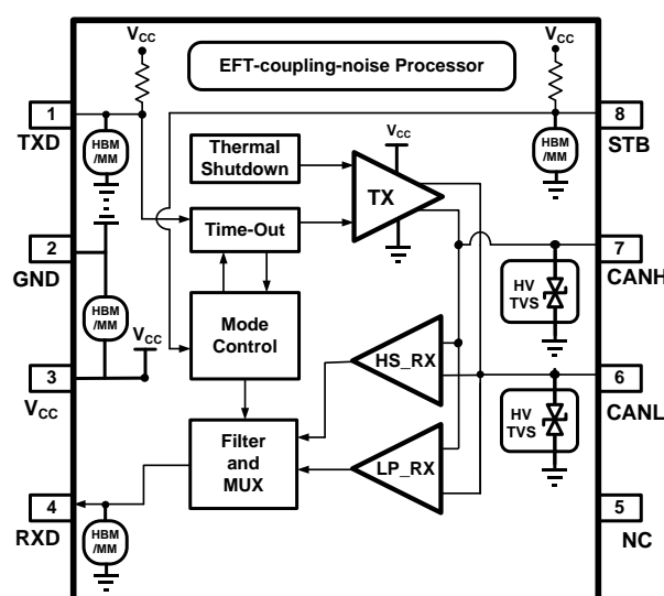
Functional Block of AZKN9215P
