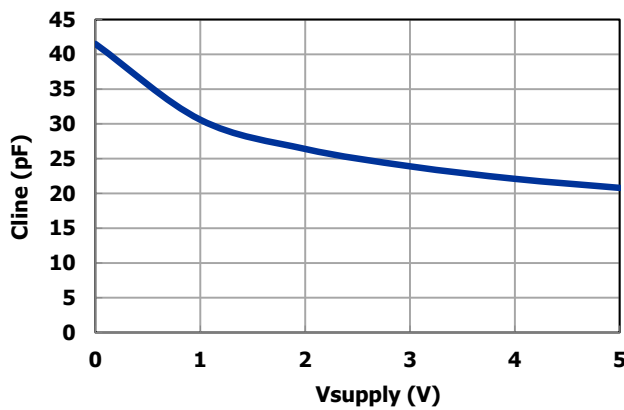
Figure 3. Line Capacitance versus Applied Voltage (typical values).
