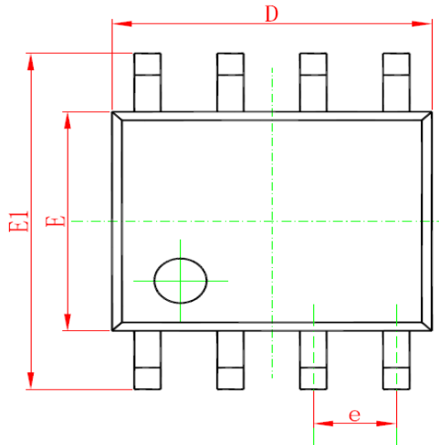
SOP-8L PACKAGE DIAGRAMS TOP VIEW
