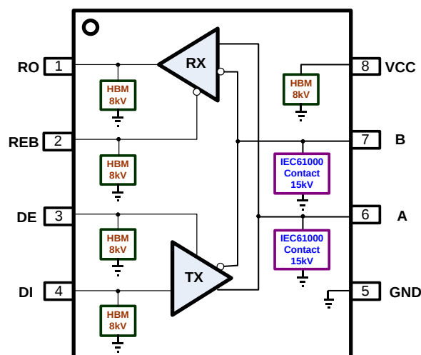
Functional Block of AZRS3080E
