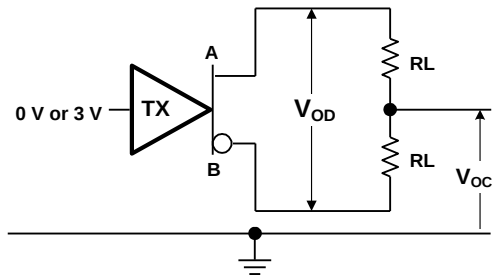
Fig.1 Transmitter DC test circuit
