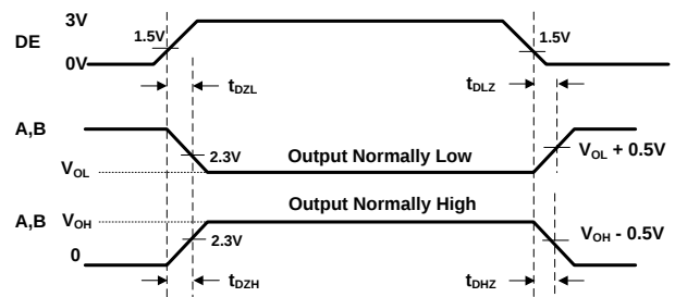
Fig.8 Transmitter Enable and Disable Times
