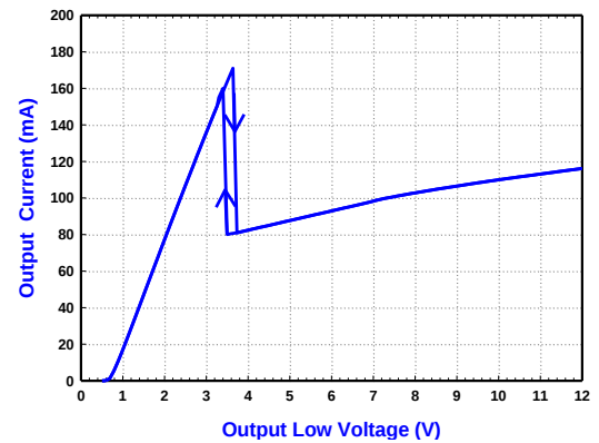
Output Current v.s. Transmitter Output Low Voltage
