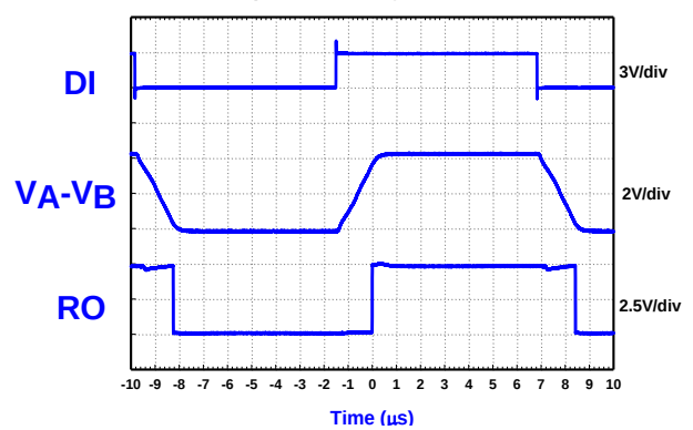
LoopBack Testing Waveform
