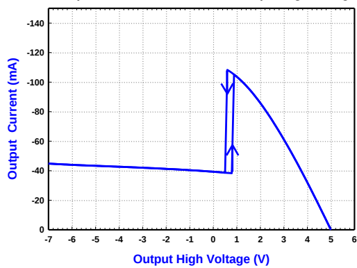
Output Current v.s. Transmitter Output High Voltage
