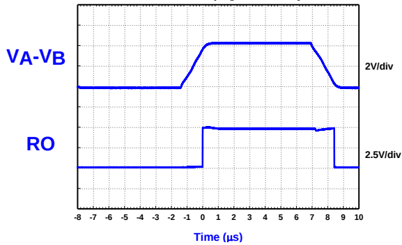
Receiver Propagation Delay
