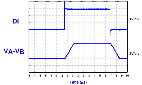
LoopBack Testing Waveform
