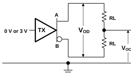
Fig.1 Transmitter DC test circuit
