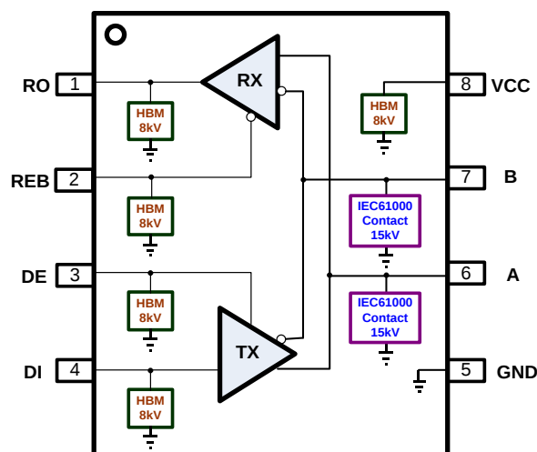
Functional Block of AZRS485E
