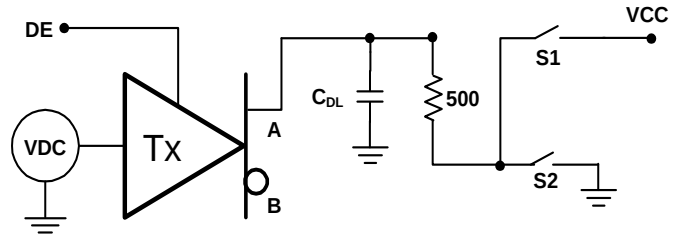
Fig.2 Transmitter timing test circuit
