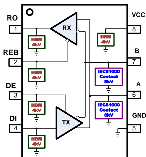
Functional Block of AZRS6605
